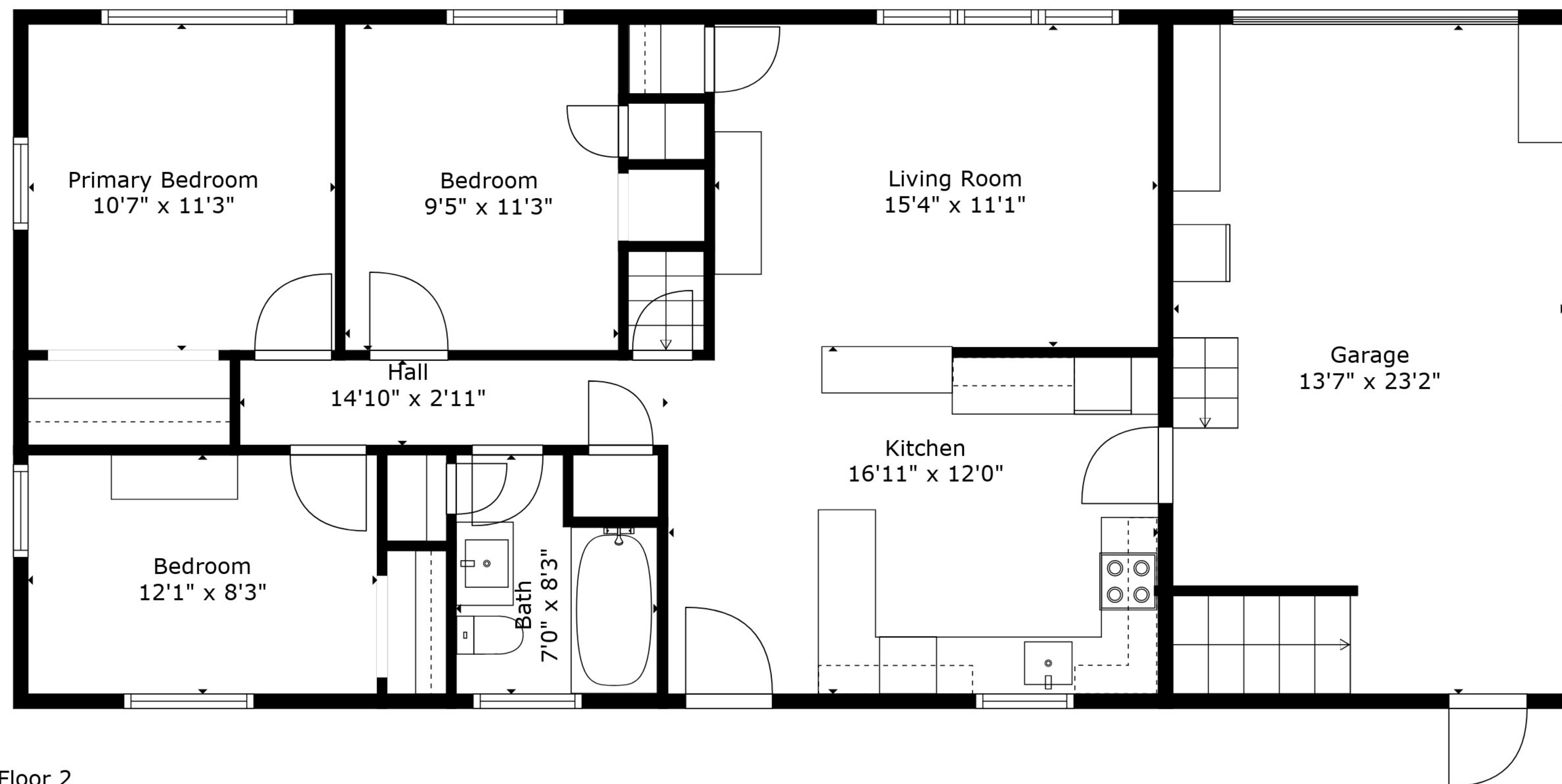
Floor 2
